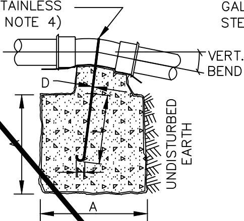
VERTICAL BLOCKING FOR 11 1/4° & 22 1/2° BENDS
