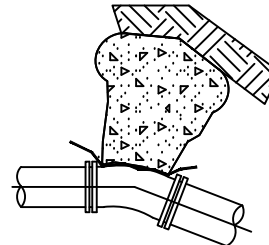
22 1/2° BEND
