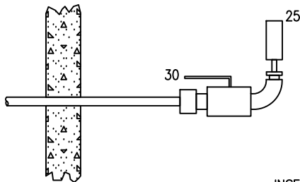
DETAIL B PRESSURE GAGE DETAIL
