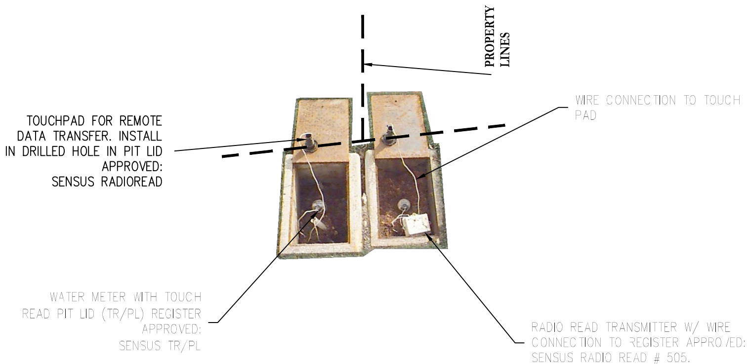
METER PIT WITH LID OPEN
