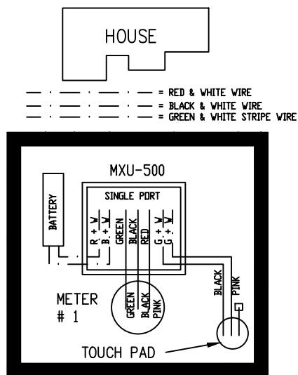
METER INSTALLATION FOR SINGLE PORT MXU
