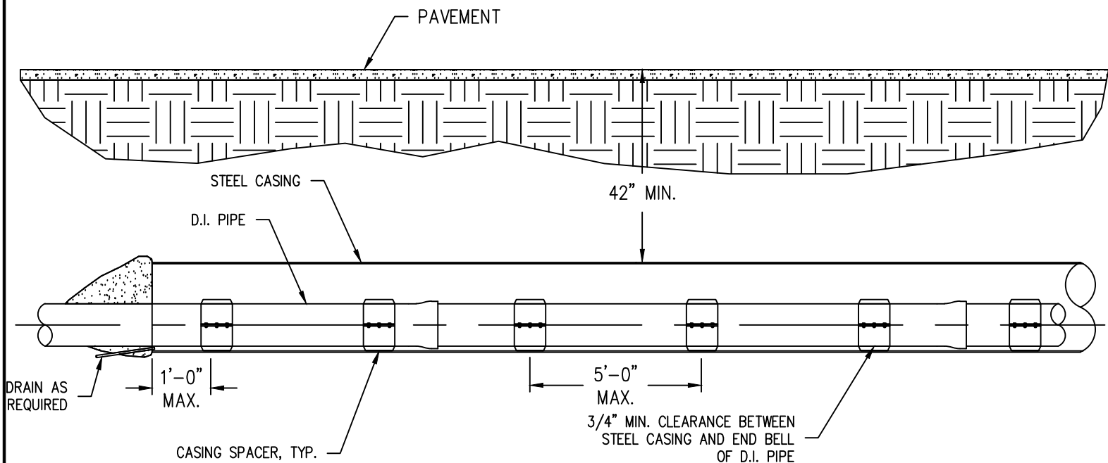
PROFILE
