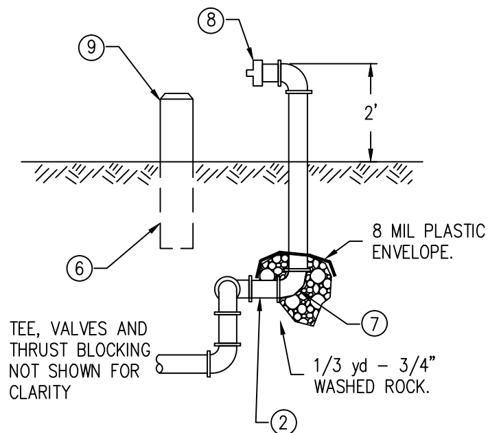
ELEVATION VIEW
