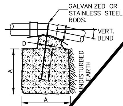
VERTICAL BLOCKING FOR 11 1/4°, 22 1/2°, & 30° BENDS
