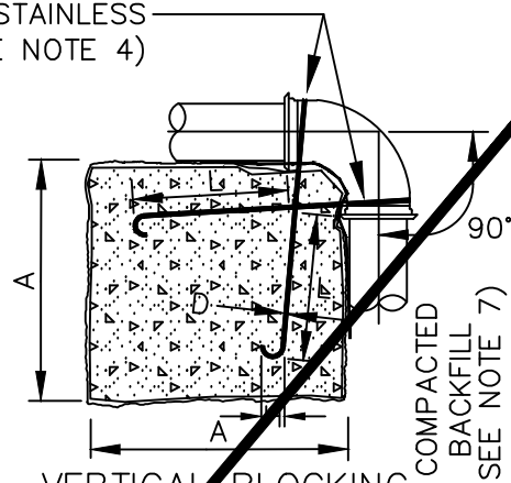
VERTICAL BLOCKING FOR 90° BENDS (SEE NOTE 6)
