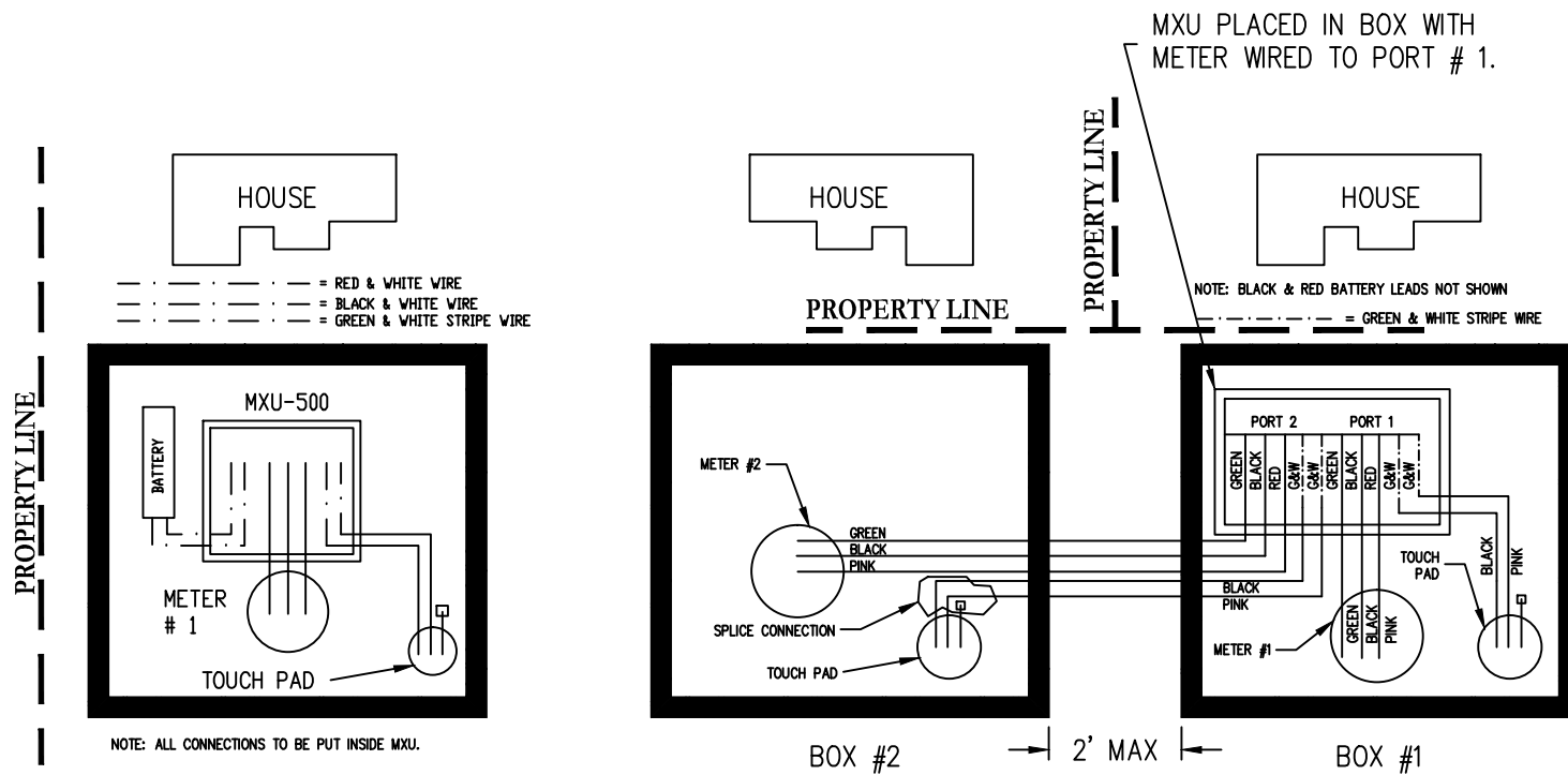
METER INSTALLATION FOR SINGLE PORT MXU
