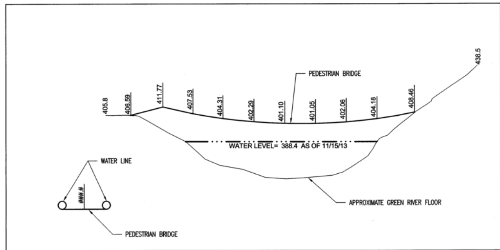
PEDESTRIAN BRIDGE PROFILE AND CROSS SECTION NOT TO SCALE
