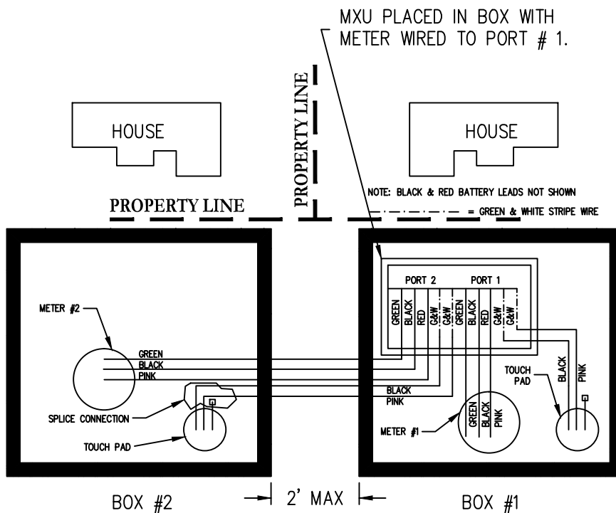
CONNECTION SCHEMATIC DOUBLE MXU (505 SERIES)
