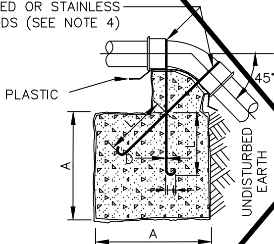
VERTICAL BLOCKING FOR 45° BENDS
