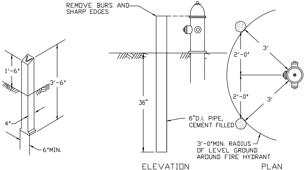
FIRE HYDRANT GUARD POST
